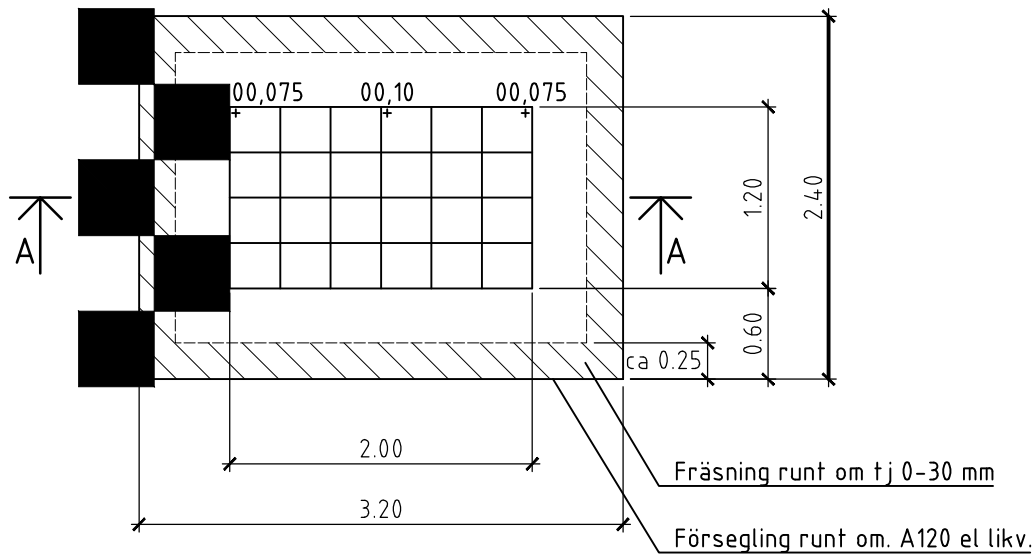
PLAN SKALA 1:50
